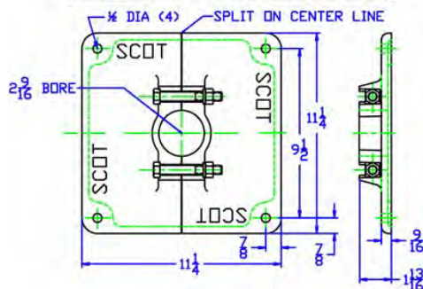
OPTIONAL MOUNTING PLATE MP11
